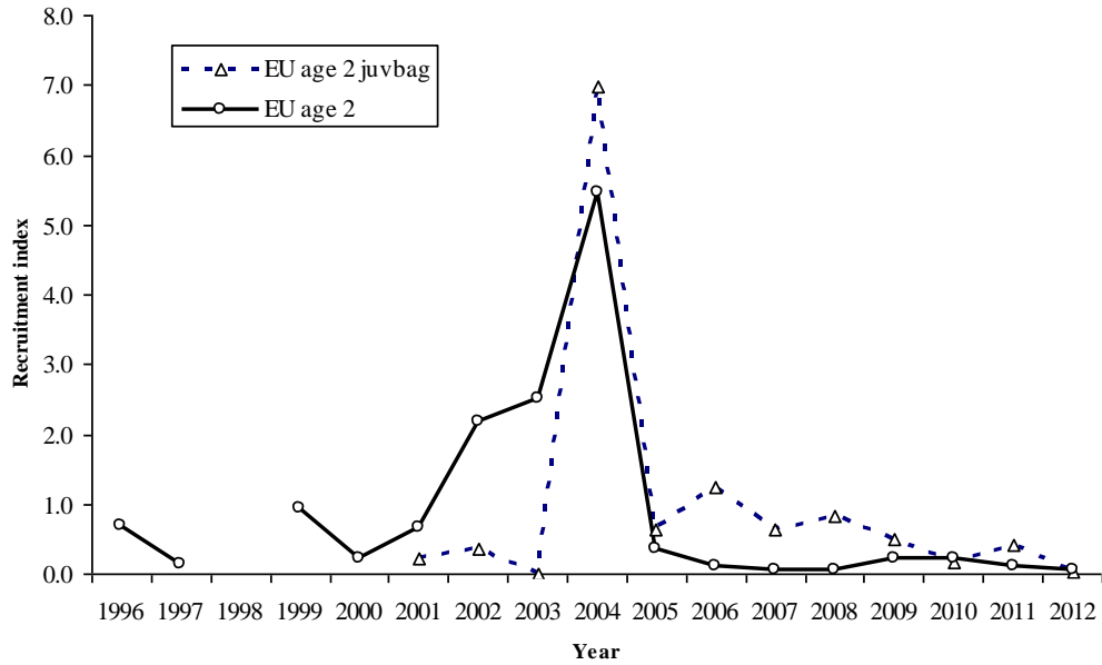
Fig. 7. Recruitment indices, abundances of age 2 in EU Survey from main gear and juvenile bag.. Each series was standardized to its mean.
