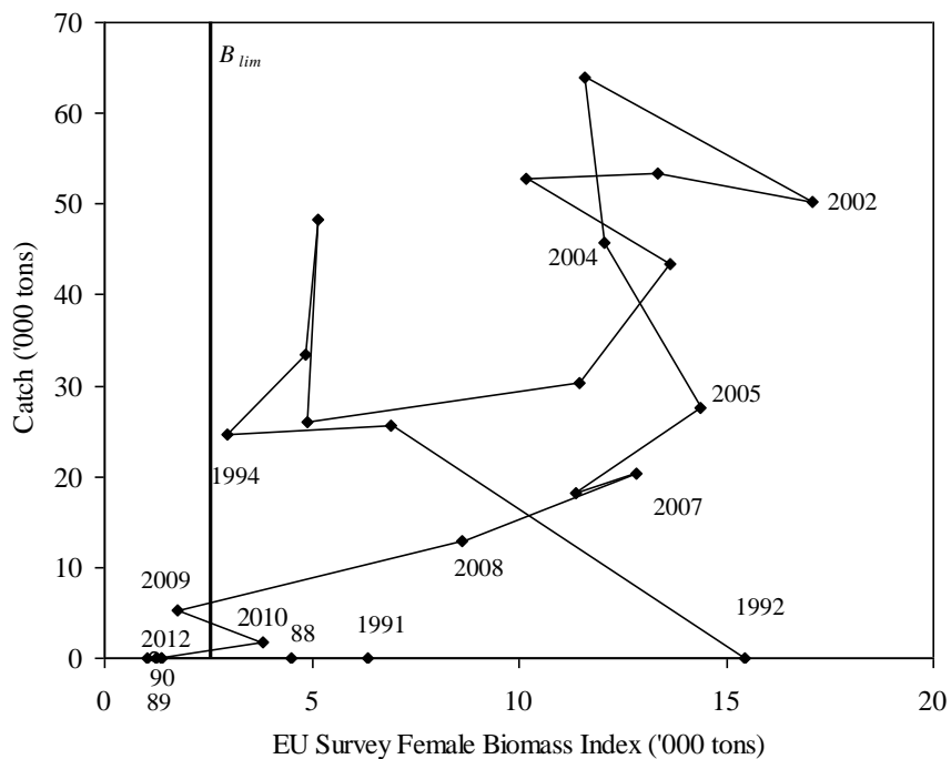
Fig. 8. Catch plotted against female biomass index from EU survey. Line denoting B_{lim} is drawn where biomass is 85% lower than the maximum point in 2002. Due to moratorium on shrimp fishery the expected catch in 2012 is 0 t.
