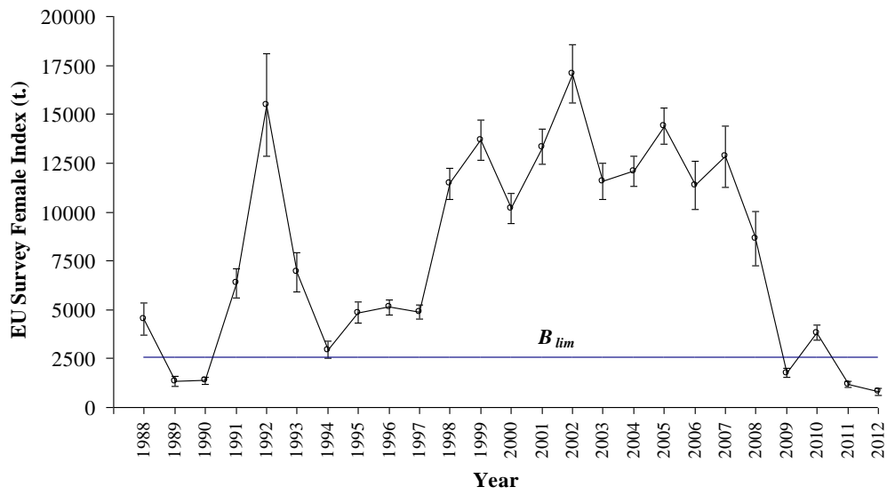
Fig. 3. Shrimp in Div. 3M: Female biomass index from EU surveys, 1988-2012.
